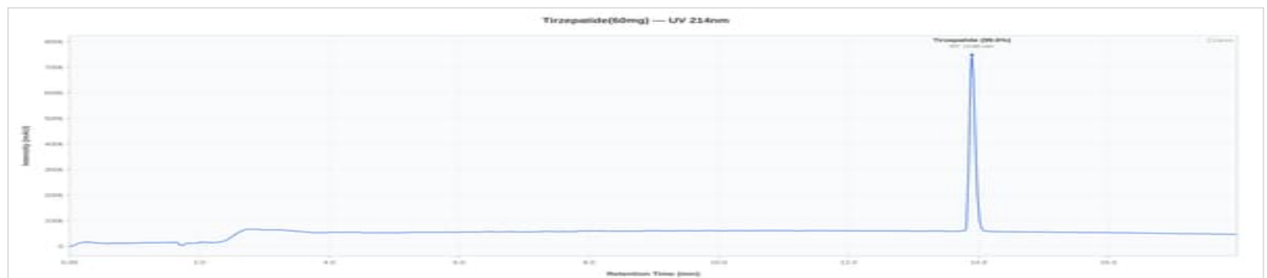
Tirzepatide 60mg - J210PC: UV Chromatogram
