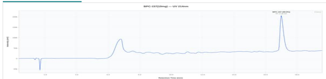
Representative chromatogram, Dedicated V0 (99.92% purity, closest to batch mean of 99.70%)
