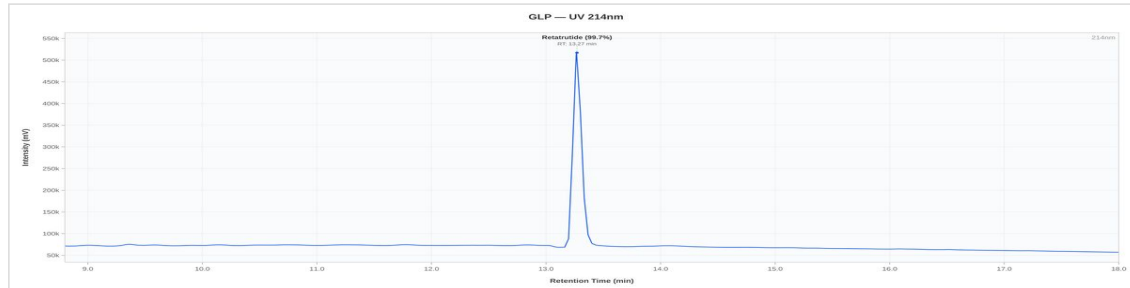
GLP 10mg - #1111: UV Chromatogram
