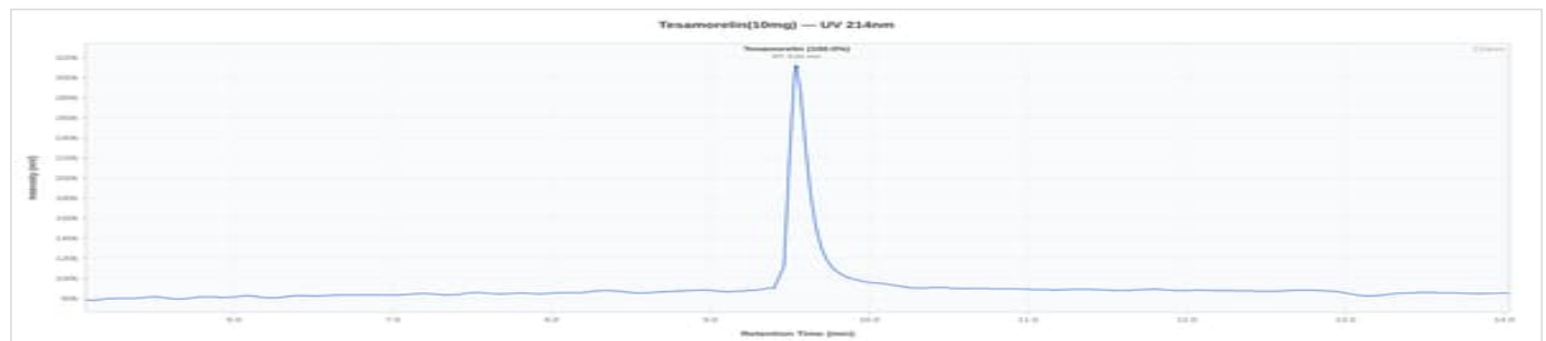
Tesamorelin 10mg - MPTA005: UV Chromatogram
