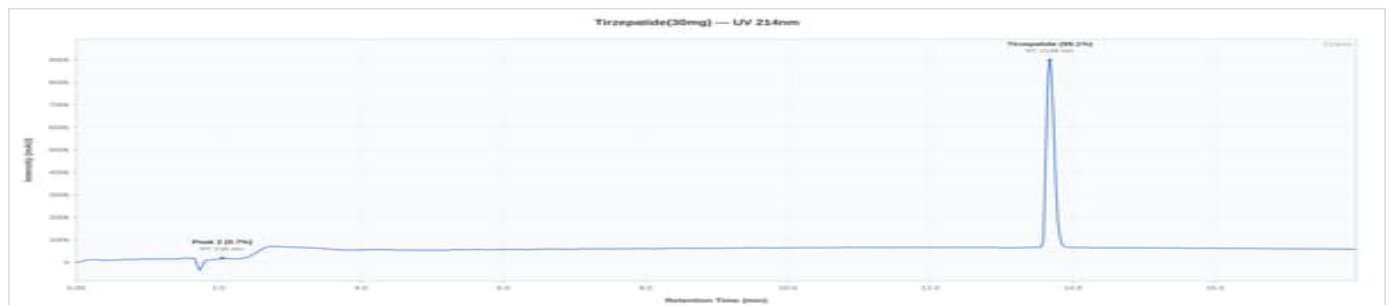
GLP-2 TZ 30mg - MPTZ008: UV Chromatogram
