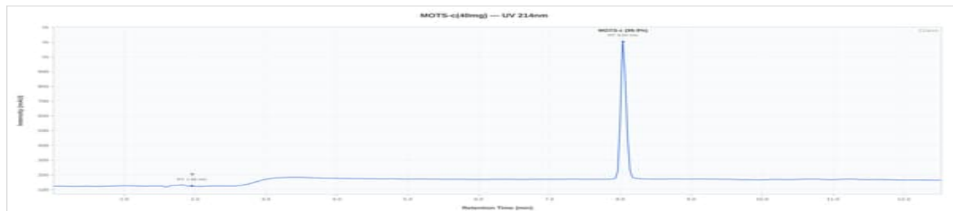
MOTS-C 40mg - MO40-2606: UV Chromatogram
