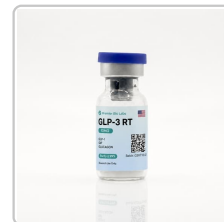
PS-R3 10mg - G3RT10-02
