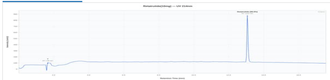
PS-R3 10mg - G3RT10-02: UV Chromatogram
