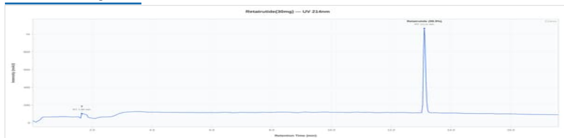
PS-R3 30mg - G3RT30-03: UV Chromatogram
