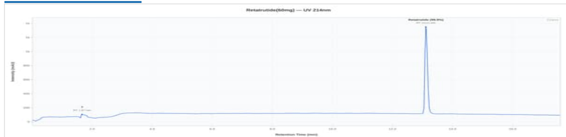
PS-R3 60mg - G3RT60-02: UV Chromatogram
