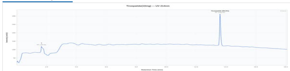
PS-T2 10mg - GTZ010-02: UV Chromatogram
