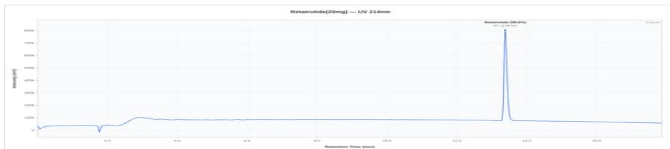
Retatrutide 20mg - VLR-RT20-0726: UV Chromatogram
