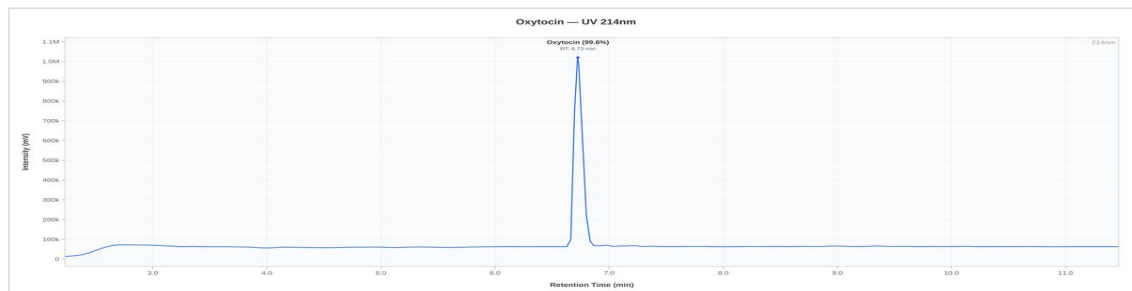
Representative chromatogram, Conformity Sample 1 (99.71% purity, closest to batch mean of 99.69%)
