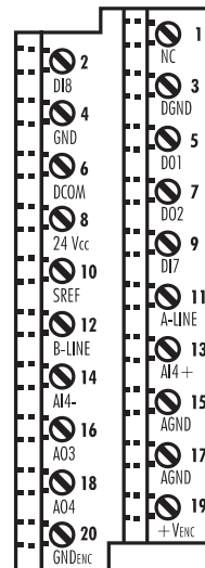
EBA line – XC4 Terminal Block description
