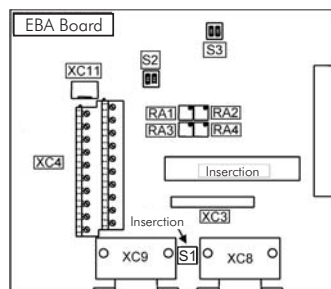
Figure 4: Configuration switches of EBA board
