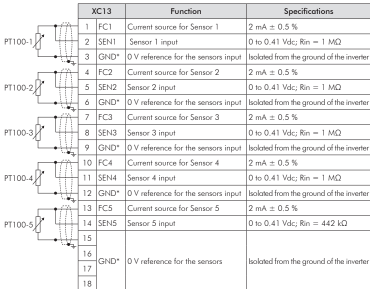
Figure 5 - Connector XC13 – IOE-02
