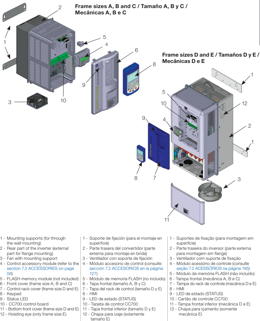
Figure A.1: Main components of the CFW700
