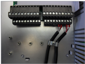
(b) Connection sample of the shield to ground
