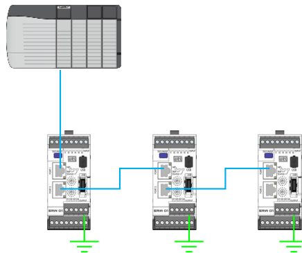
Figura 4.2: Topologia daisy chain
