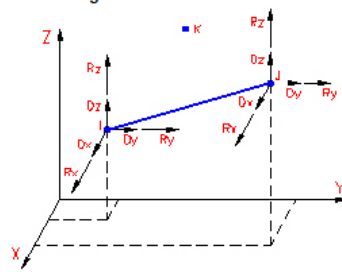
Figure 2: Beam Element Degrees-of-Freedom
