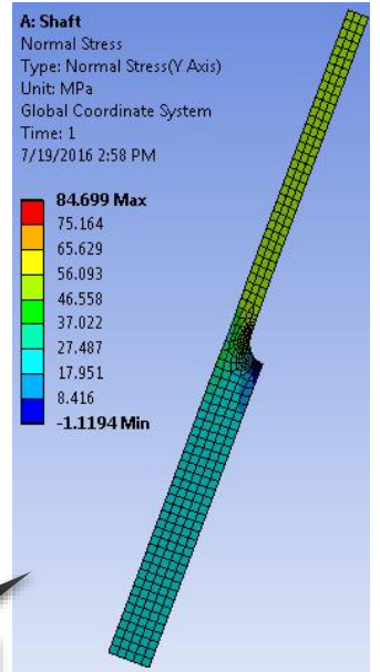
Normal Stress.
