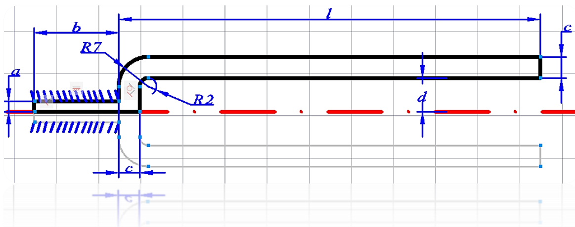
Symmetric model
