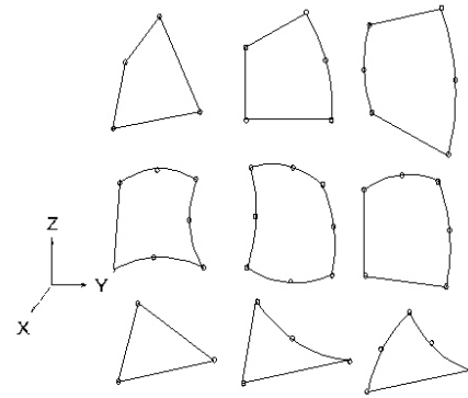
Figure 2: Typical Shell Elements
